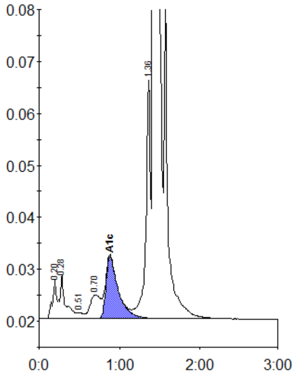
Peak table - ID: 10619097
